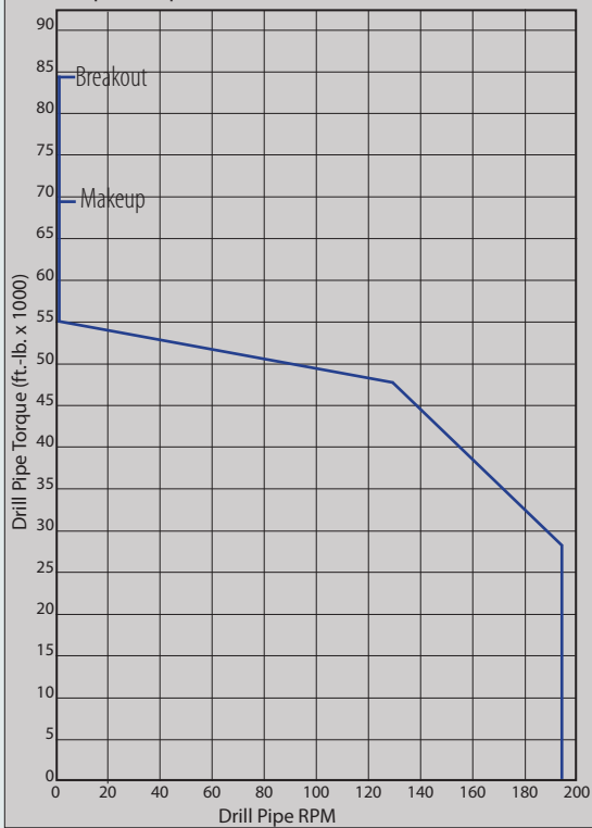
Performance Curve 750 TON ECIX 1350 HP TOP DRIVE Torque vs. Speed - 18.61:1 Gear Ratio (Standard)
